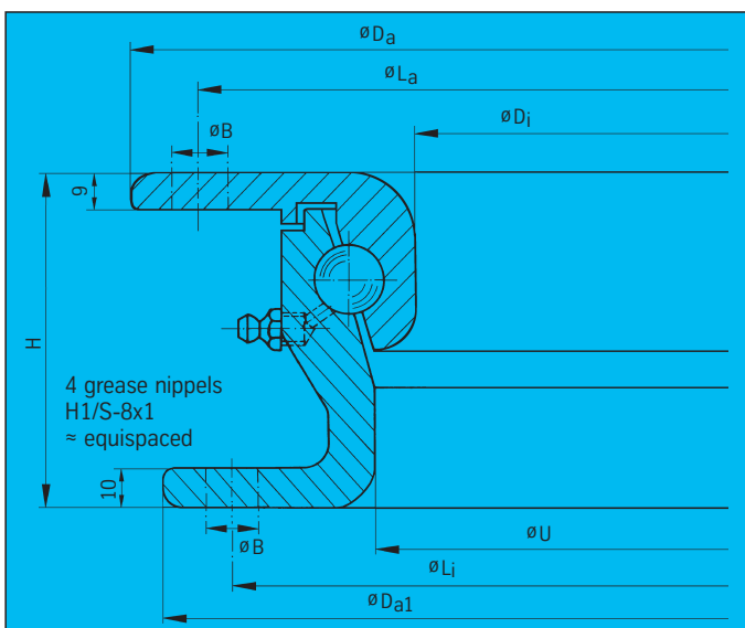
Type 80 capable for two- and three-axle trailers of over 25 km/h
